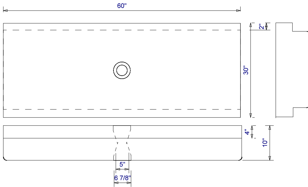
Conical Support Column
