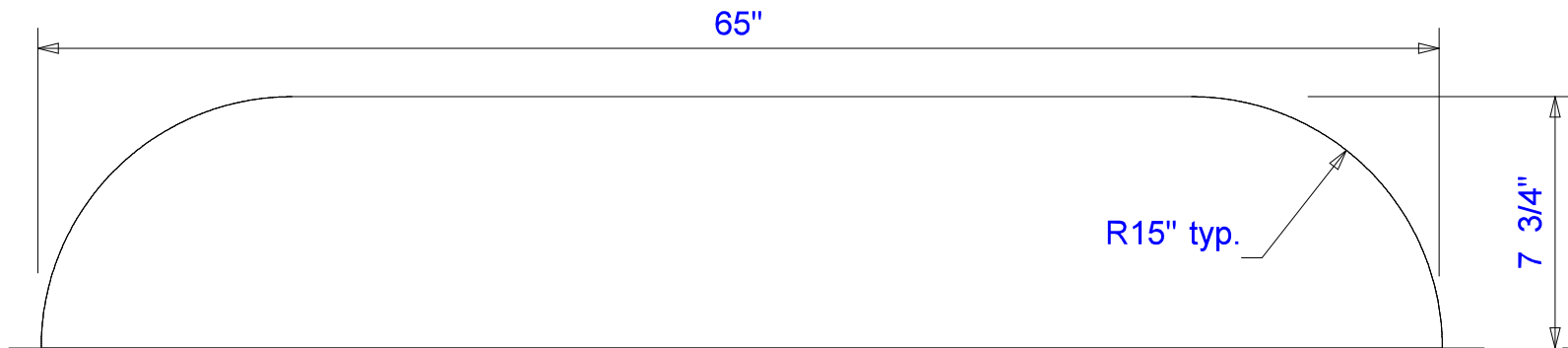
Side View
