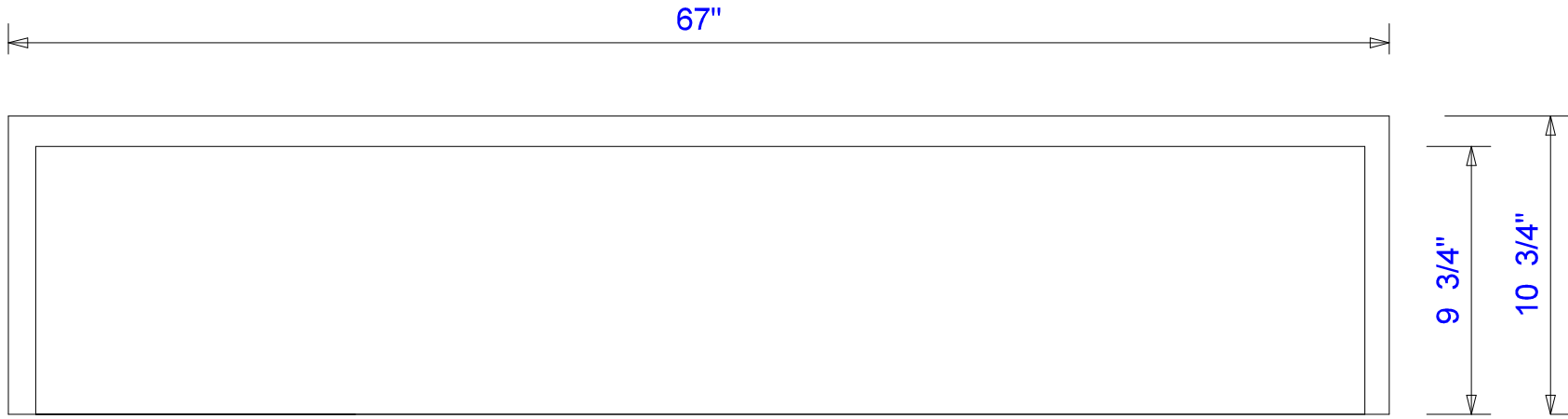
Top View
